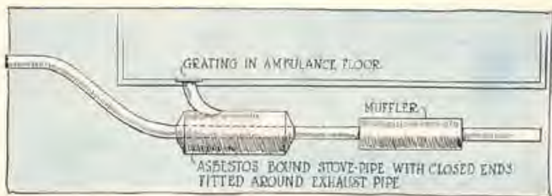
Method of heating Ford ambulance
